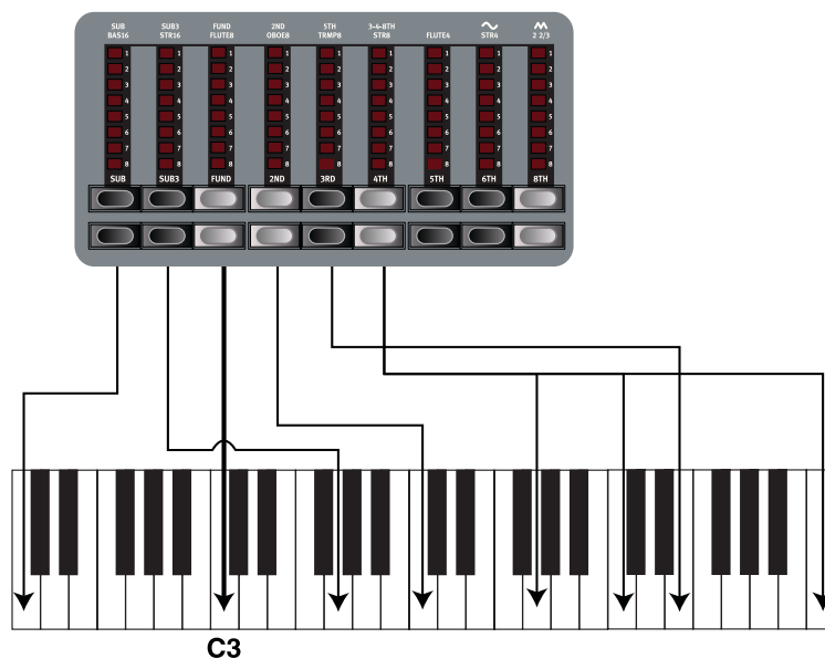
In the illustration above we have chosen C3 as our reference note. The FUND drawbar is considered the basic (fundamental) harmonic in the organ sound. The arrows point at the respective note that each drawbar represents when C3 is our reference note.
