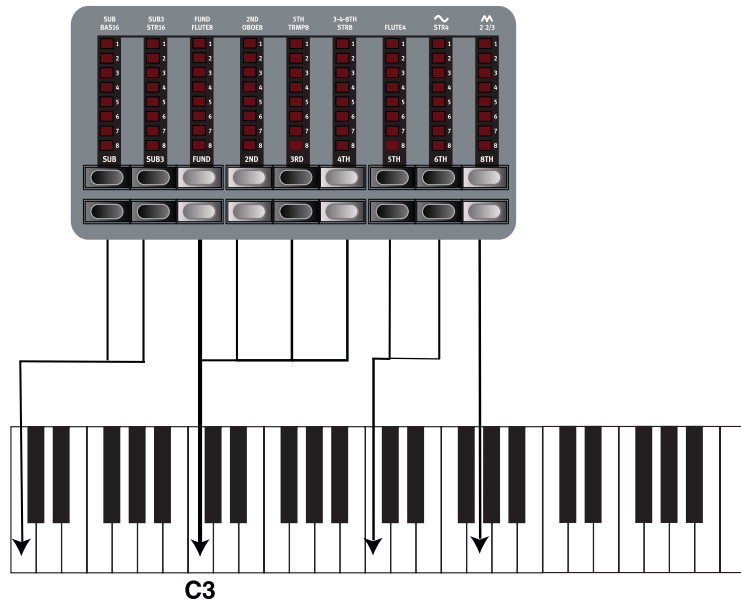
In the illustration above we have chosen C3 as our reference note. The four ‘Register selectors correspond to the fundamental harmonic (but with different tonal characteristics). The arrows point at the respective note that each drawbar represents when C3 is our reference note.
